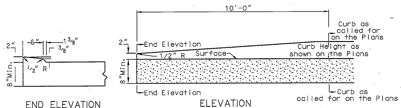
STANDARD CURB TAPER CLASS II
