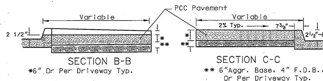
SIDEWALK AND CURB TREATMENT AT DRIVEWAYS
